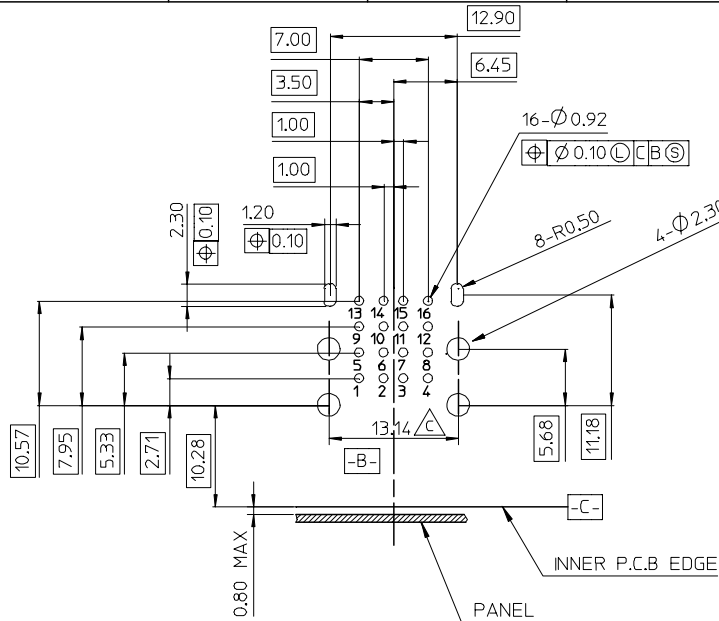
RECOMMENDED P.C.B. LAYOUT (2) (THICKNESS=1.6MM) (GENERAL TOLERANCE: ±0.05MM)
